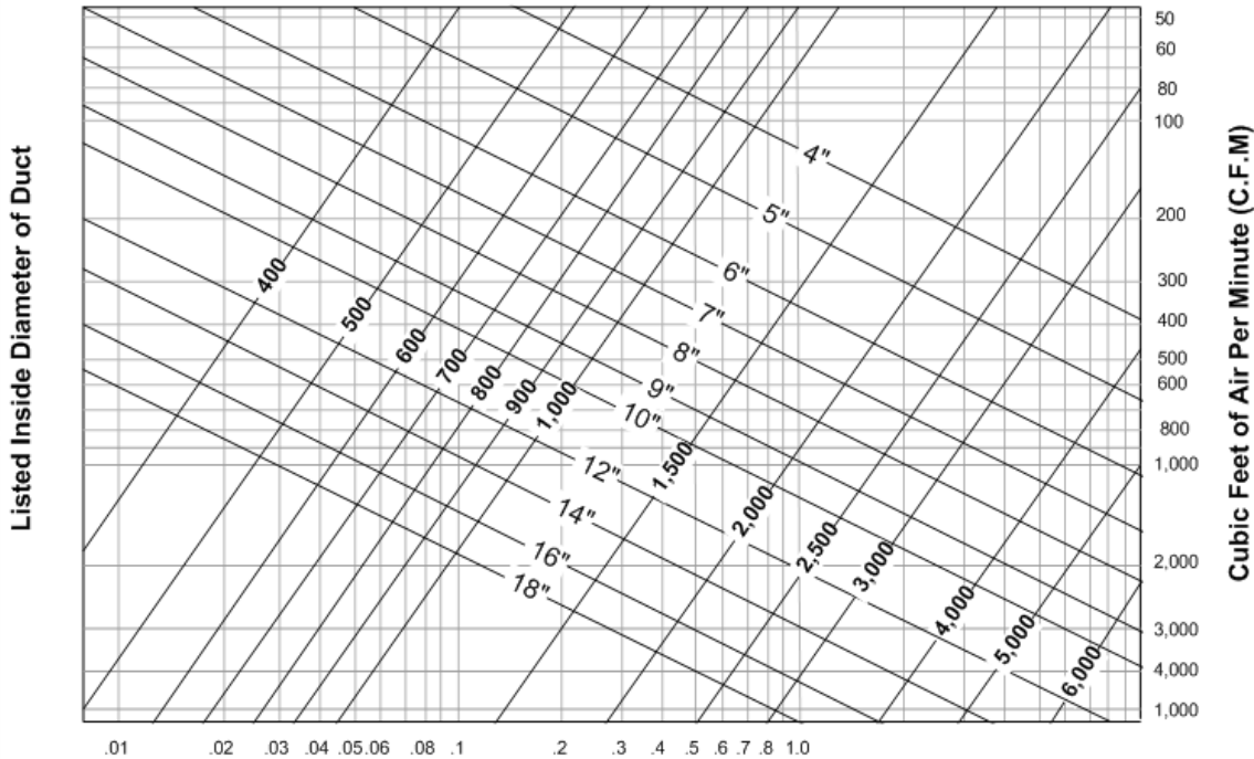
Friction Loss in Inches of Water Per 100 Feet
