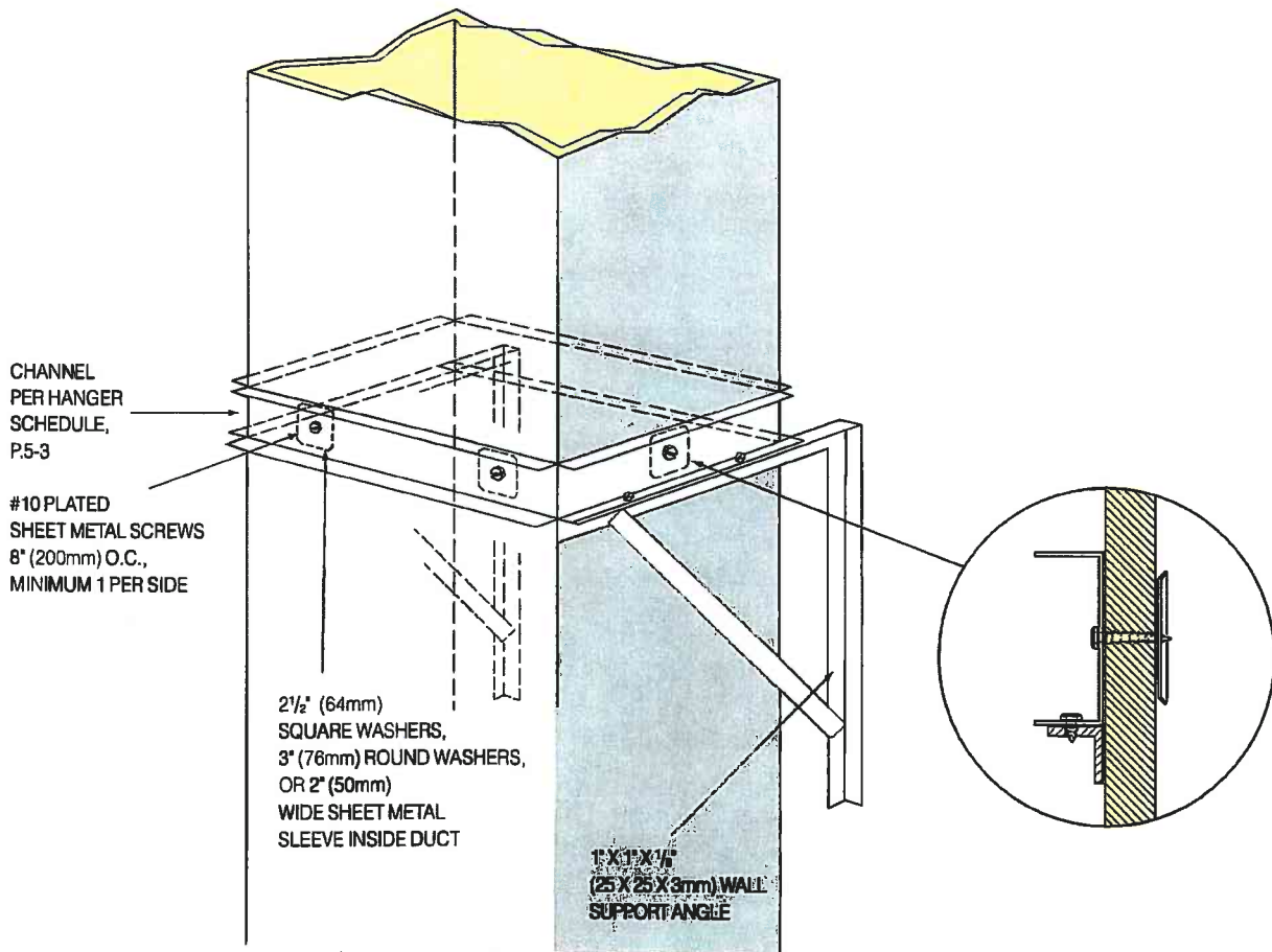
Fig. 6-7. Vertical riser support.
